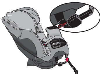
Rear-facing Belt Path
